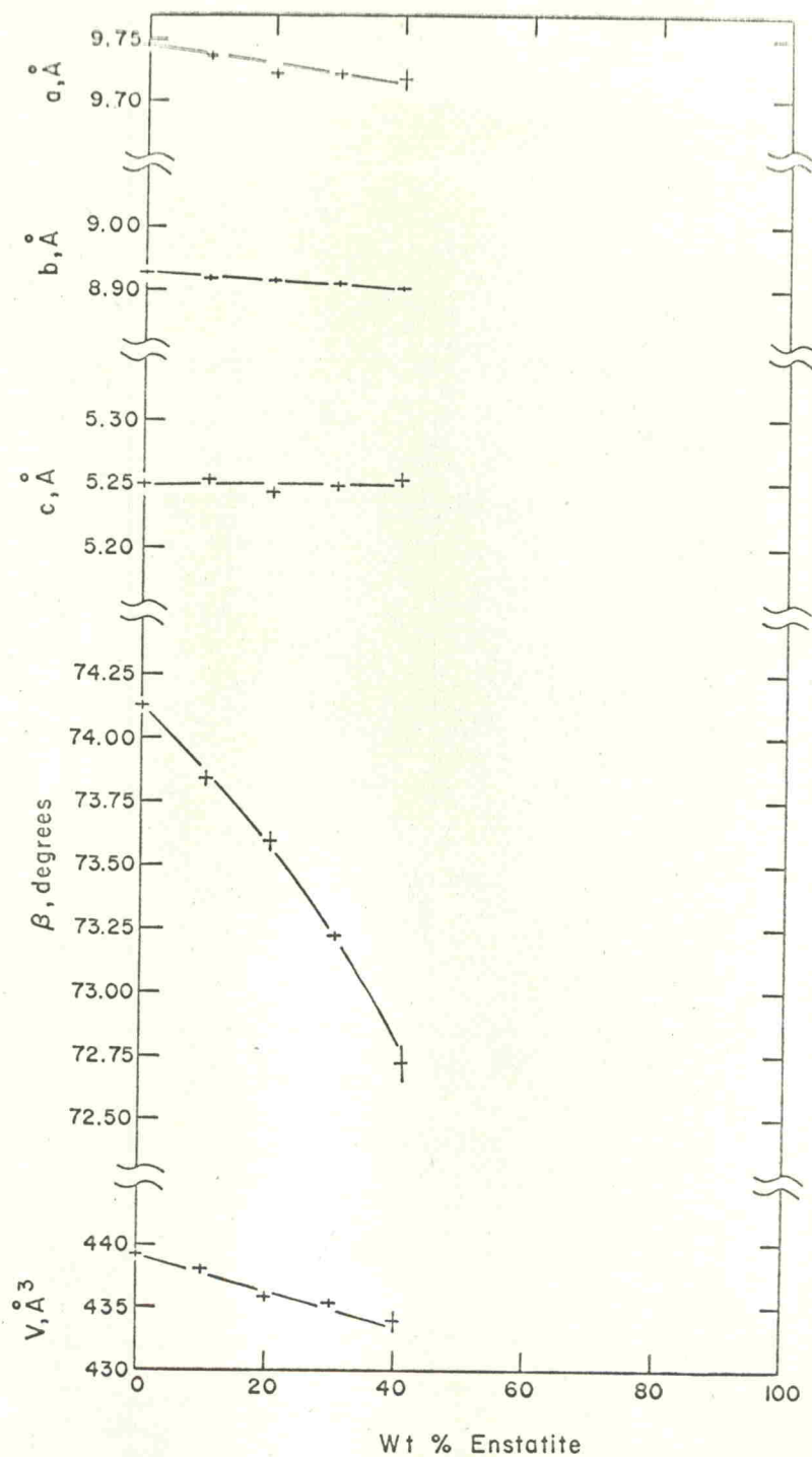
Fig. 5. Unit-cell parameters along the join diopside-enstatite.
